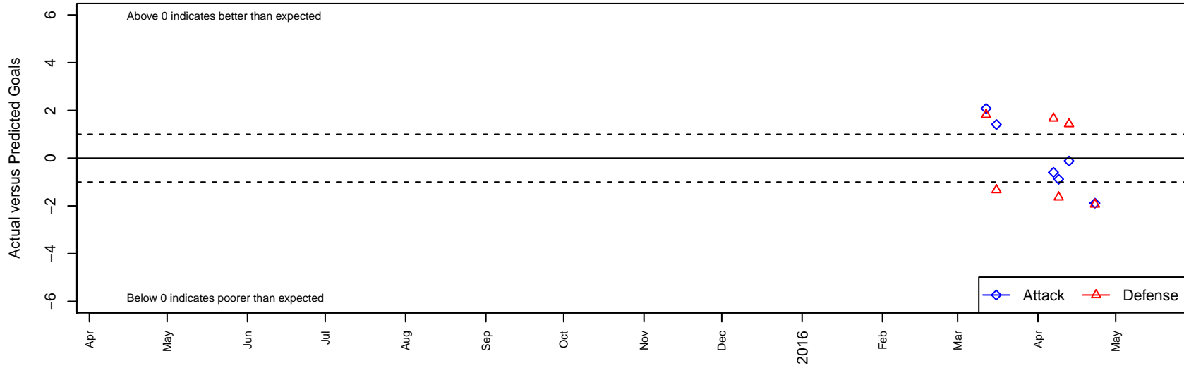
Boise Nationals SC Sao Paulo G00 Dots are actual minus expected GF (blue circles) and GA (red triangles). Blue line is smoothed change in attack strength. Red is smoothed change in defense strength.
